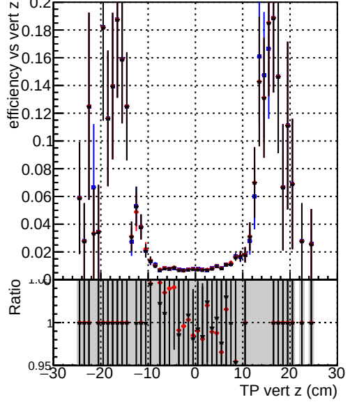
Efficiency vs vert z —●— DQM_original_step2_ttbar-phase1-newgeom —●— DQM_pixelCPE_step2_ttbar-phase1-newgeom —●— DQM_pixelCPEAndChi2_step2_ttbar-phase1-newgeom
