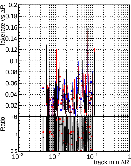
Fake rate vs \Delta R(\text{track, jet}) Legend: DQM_original_step2_ttbar-phase1-newgeom (blue line with dots) DQM_pixelCPE_step2_ttbar-phase1-newgeom (red line with dots) DQM_pixelCPEAndChi2_step2_ttbar-phase1-newgeom (black line with dots)
