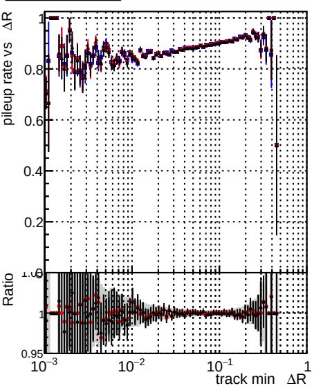
Legend: DOM CKFFit 1000evt (blue line with dots), DOM CKFREFitOLD 1000evt (red line with dots), DOM MkFitREFitOLD 1000evt (black line with dots)
