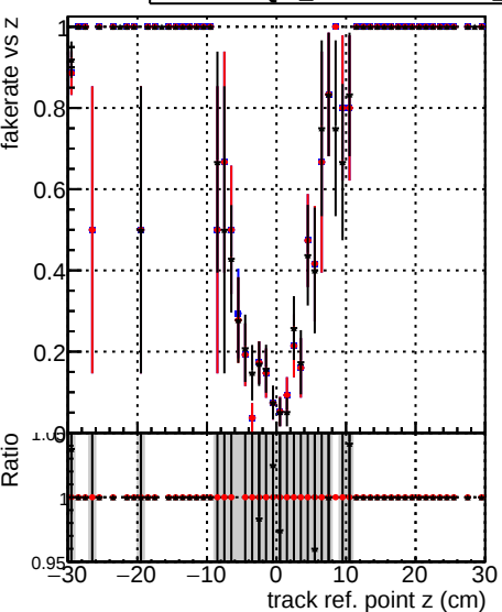
Fake rate vs z Legend: DOM CKFFit 1000evt (blue line with circles) DOM CKFREFitOLD 1000evt (red line with circles) DOM MkFitREFitOLD 1000evt (black line with circles)
