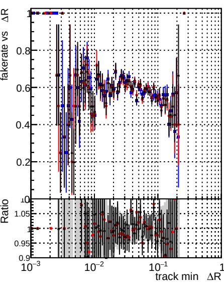
Legend: DOM CKFFit 1000evt (blue line with dots) DOM CKFREFit 1000evt (red line with dots) DOM MkFitREFit 1000evt (black line with dots)
