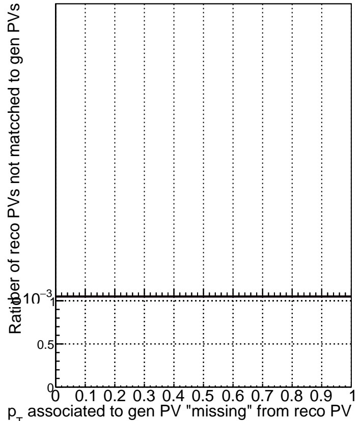
RecoPVAssoc2GenPVnotmatched_missing
