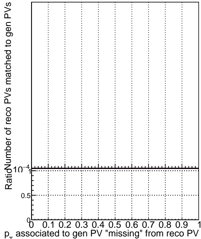
RecoPVAssoc2GenPVmatched_missing
