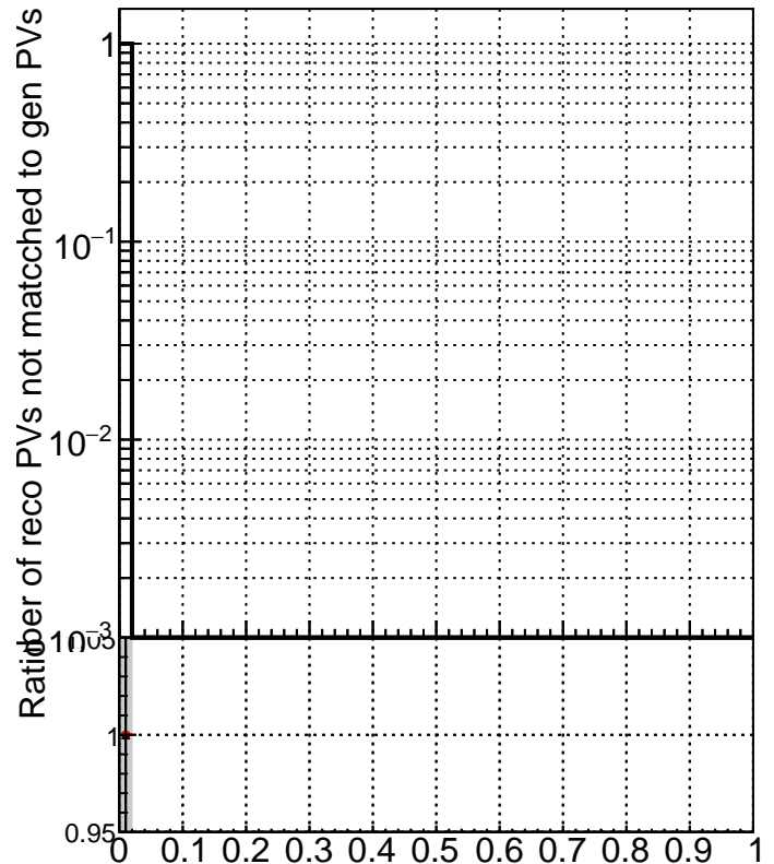
RecoPVAssoc2GenPVNotMatched_Purity
