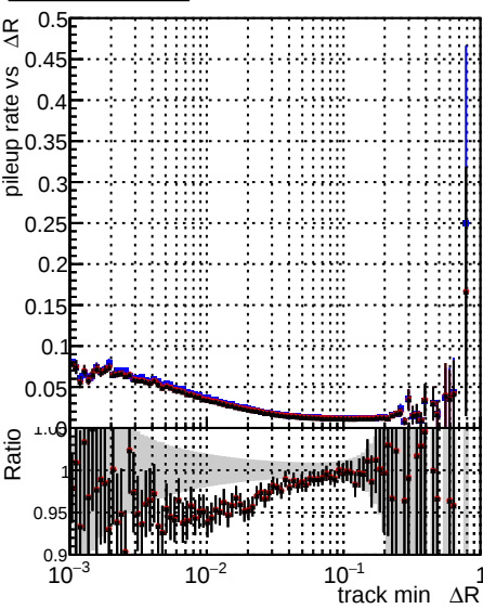
Legend: - blue line with error bars: DQM original originalvector 1000evt - red line with error bars: DQM fit cpeOK_SORTRZ2_TESTOUTLIER5_1000evt - black line with error bars: DQM fit cpeOK_SORTRZ2_TESTOUTLIER6_1000evt
