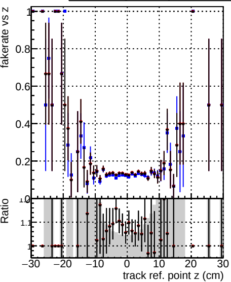
Fake rate vs —●— DOM original originalvector 1000evt —●— DOM fit cpeOK SORTR22 TESTOUTLIER5 1000evt —●— DOM fit cpeOK SORTR22 TESTOUTLIER6 1000evt
