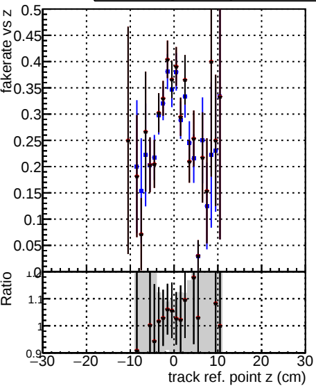
Fake rate vs track ref. point z (cm) Legend: DOM original originalvector 1000evt (blue line with circles) DOM fit cpeOK SORTRZ2 TESTOUTLIER5 1000evt (red line with circles) DOM fit cpeOK SORTRZ2 TESTOUTLIER6 1000evt (black line with circles)
