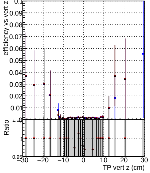
Efficiency vs. TP vert z (cm) Legend: - DQM_original_originalvector_1000evt (blue line with points) - DQM_fit_cpeOK_SORTRZ2_TESTOUTLIER5_1000evt (red line with points) - DQM_fit_cpeOK_SORTRZ2_TESTOUTLIER6_1000evt (black line with points)
