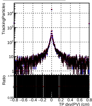
N of sim → DQM_fit_cpeOK_SORTI
