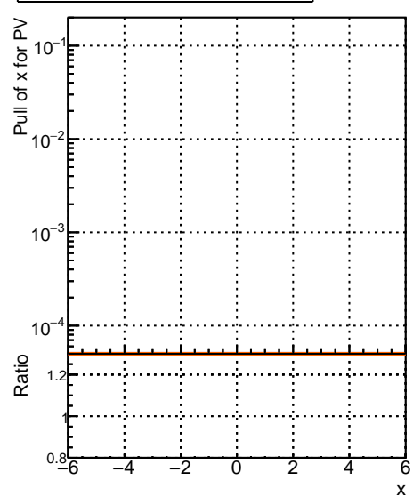
RecoPVAssoc2GenPVMatched_PulIX
