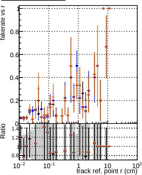
Fake rate vs vertpos DOM original original vector 1000evt DOM fit cpeak sort rzz test outlier 5 1000evt DOM fit cpeak sort rzz test outlier 8 gets 1000evt
