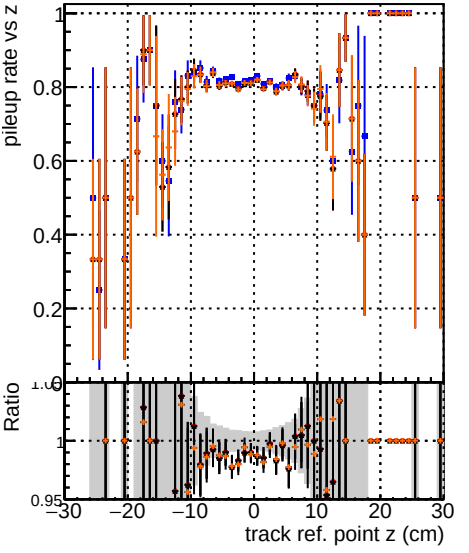
Fake rate vs z Duplicates Rate vs z Pileup rate vs z Legend: DOM original (blue squares), DOM fit (black circles), DOM fit peak (red circles), DOM fit peak sort (orange circles), DOM fit peak sort rzz (black circles), DOM fit peak sort rzz test outlier (black circles), DOM fit peak sort rzz test outlier gets 1000evt (orange circles).
