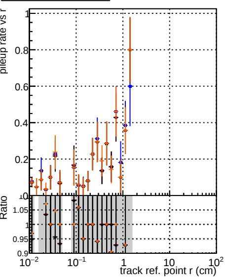
—•— DOM original original vector 1000evt —•— DOM fit cpeak SORT RZ2 TESTOUTLIER5 1000evt —•— DOM fit cpeak SORT RZ2 TESTOUTLIER6 1000evt —•— DOM fit cpeak SORT RZ2 TESTOUTLIER8 gets 1000evt
