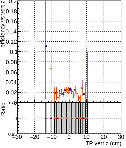
Efficiency vs vertpos Legend: DOM original originalvector 1000evt DOM_fit_cpeOK_SORTRZ2_TESTOUTLIER5_1000evt DOM_fit_cpeOK_SORTRZ2_TESTOUTLIER6_1000evt DOM_fit_cpeOK_SORTRZ2_TESTOUTLIER6_getS_1000evt
