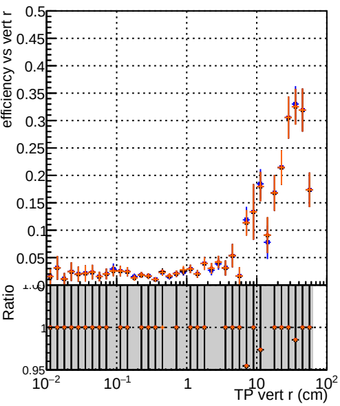
Efficiency vs vertpos Legend: DOM original originalvector 1000evt DOM_fit_cpeOK_SORTRZ2_TESTOUTLIER5_1000evt DOM_fit_cpeOK_SORTRZ2_TESTOUTLIER6_1000evt DOM_fit_cpeOK_SORTRZ2_TESTOUTLIER6_getS_1000evt
