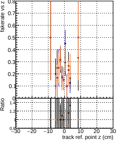
Fake rate vs verpos DOM original original vector 1000evt DOM fit peak sorted by test outlier 1000evt DOM fit peak sorted by test outlier gets 1000evt
