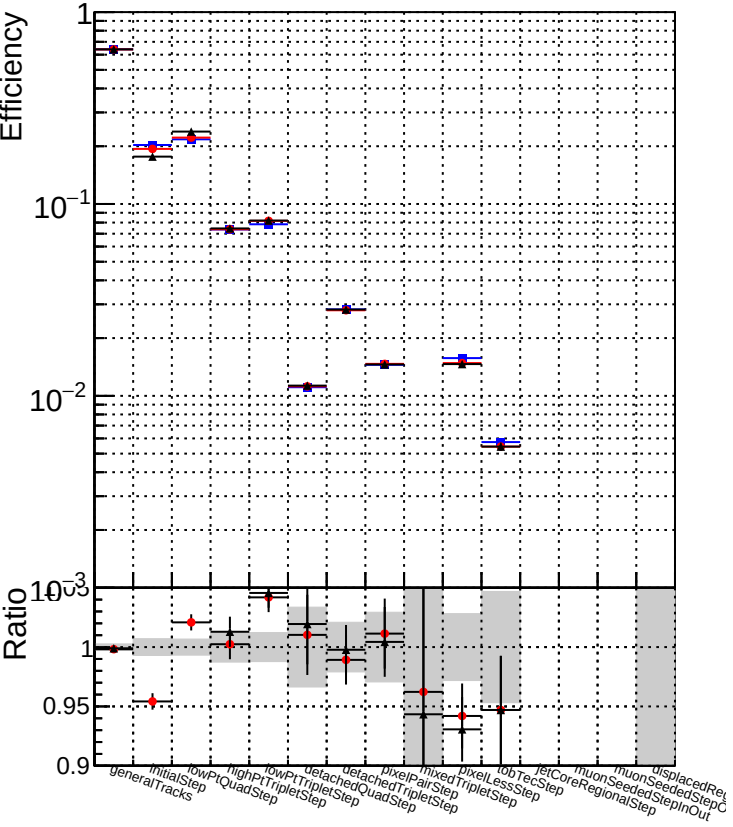
DQM_original_step2_ttbar-phase1-newgeom DQM_pixelCPE_step2_ttbar-phase1-newgeom DQM_pixelCPEChi2OR2_step2_ttbar-phase1-newgeom
