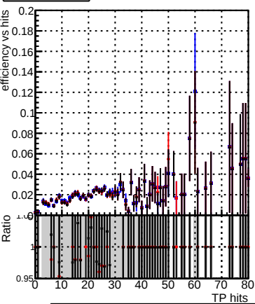
Efficiency vs TP hits Legend: DQM_original_step2_ttbar-phase1-newgeom (blue line with markers) DQM_pixelCPE_step2_ttbar-phase1-newgeom (red line with markers) DQM_pixelCPEChi2OR2_step2_ttbar-phase1-newgeom (black line with markers)
