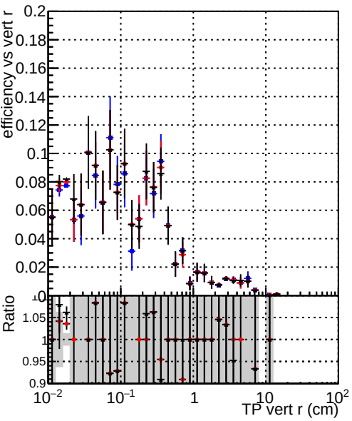
Efficiency vs TP vert r (cm) Legend: DQM_original_step2_ttbar-phase1-newgeom DQM_pixelCPE_step2_ttbar-phase1-newgeom DQM_pixelCPEChi2OR2_step2_ttbar-phase1-newgeom
