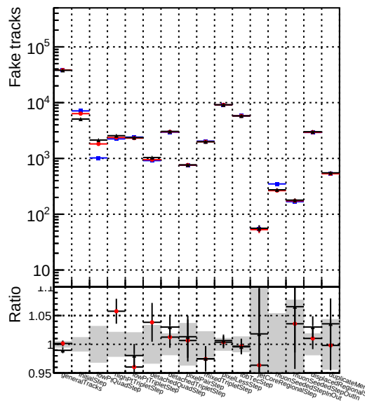
Number Legend 1 DQM_pixelCPE_step2_ttbar-phase1-newgeom 2 DQM_pixelCPEChi2OR2_step2_ttbar-phase1-newgeom
