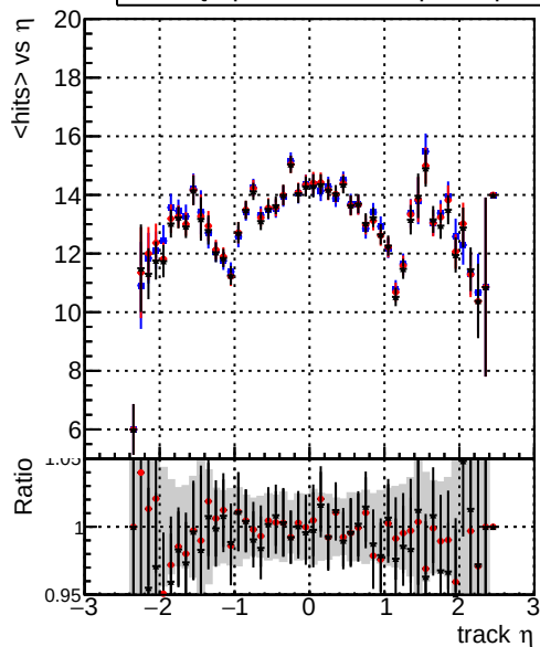
mean hits vs \eta — DQM_original_step2_ttbar-phase1-newgeom — DQM_pixelCPE_step2_ttbar-phase1-newgeom — DQM_pixelCPEChi2OR2_step2_ttbar-phase1-newgeom
