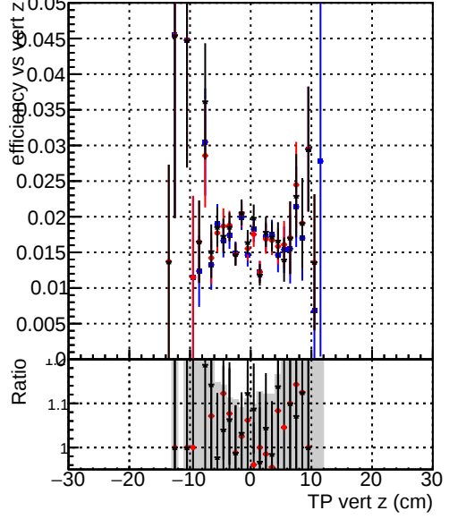
Efficiency vs vert z — DQM_original_step2_ttbar-phase1-newgeom — DQM_pixelCPE_step2_ttbar-phase1-newgeom — DQM_pixelCPEChi2OR2_step2_ttbar-phase1-newgeom
