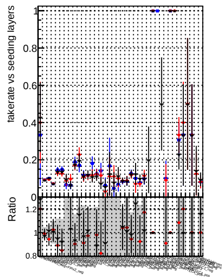
Fake rate vs. DOM original_step2_tbar-phase1-newgeom DOM CPE_step2_tbar-phase1-newgeom DOM pixe/CPEchizOR2_step2_tbar-phase1-newgeom
