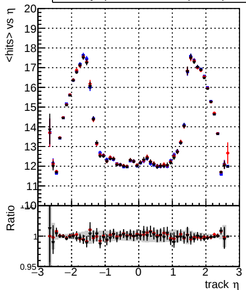
mean hits vs \eta — DQM_original_step2_ttbar-phase1-newgeom — DQM_pixelCPE_step2_ttbar-phase1-newgeom — DQM_pixelCPEChi2OR2_step2_ttbar-phase1-newgeom
