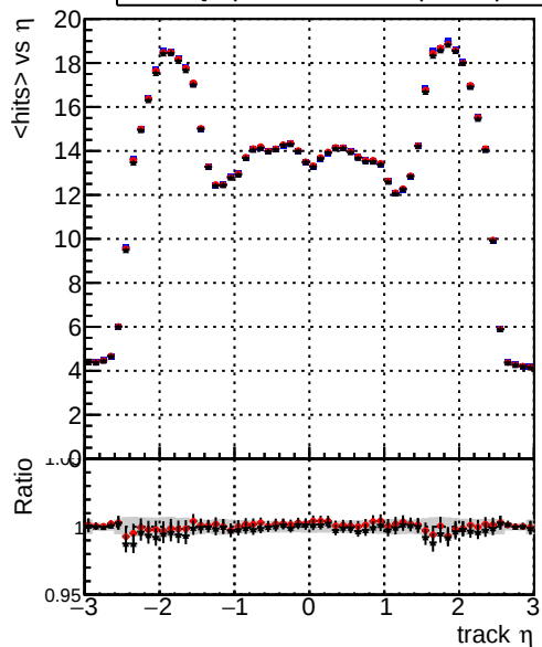
mean hits — DQM_original_step2_ttbar-phase1-newgeom — DQM_pixelCPE_step2_ttbar-phase1-newgeom — DQM_pixelCPEChi2OR2_step2_ttbar-phase1-newgeom
