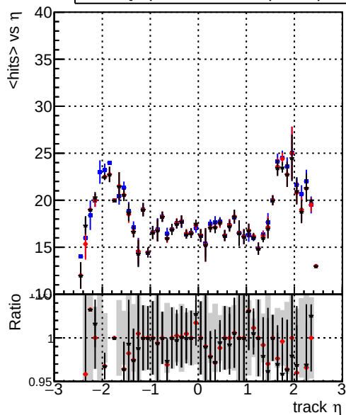
mean hits — DQM_original_step2_ttbar-phase1-newgeom — DQM_pixelCPE_step2_ttbar-phase1-newgeom — DQM_pixelCPEChi2OR2_step2_ttbar-phase1-newgeom
