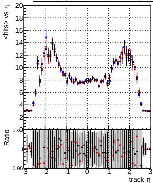
mean hits vs \eta — DQM_original_step2_ttbar-phase1-newgeom — DQM_pixelCPE_step2_ttbar-phase1-newgeom — DQM_pixelCPEChi2OR2_step2_ttbar-phase1-newgeom
