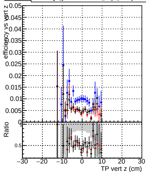
Efficiency vs. TP vert z DQM_original_step2_ttbar-phase1-newgeom DQM_pixelCPE_step2_ttbar-phase1-newgeom DQM_pixelCPEChi2OR2_step2_ttbar-phase1-newgeom
