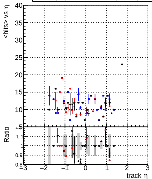
— DQM_original_step2_ttbar-phase1-newgeom — DQM_pixelCPE_step2_ttbar-phase1-newgeom — DQM_pixelCPEChi2OR2_step2_ttbar-phase1-newgeom mean hits
