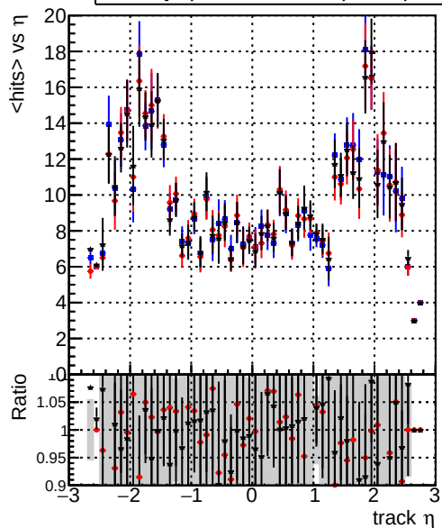
mean hits vs \eta Legend: - DQM_original_step2_ttbar-phase1-newgeom (blue line) - DQM_pixelCPE_step2_ttbar-phase1-newgeom (red line) - DQM_pixelCPEChi2OR2_step2_ttbar-phase1-newgeom (black line)
