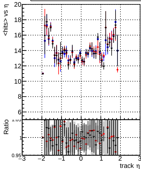
mean hit — DQM_original_step2_ttbar-phase1-newgeom — DQM_pixelCPE_step2_ttbar-phase1-newgeom — DQM_pixelCPEChi2OR2_step2_ttbar-phase1-newgeom
