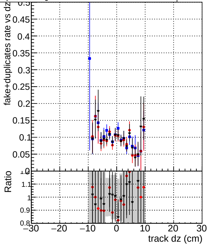
Legend for the bottom plot: DQM_original_step2_ttbar-phase1-newgeom (Blue squares) DQM_pixelCPE_step2_ttbar-phase1-newgeom (Red circles) DQM_pixelCPEChi2OR2_step2_ttbar-phase1-newgeom (Black triangles)
