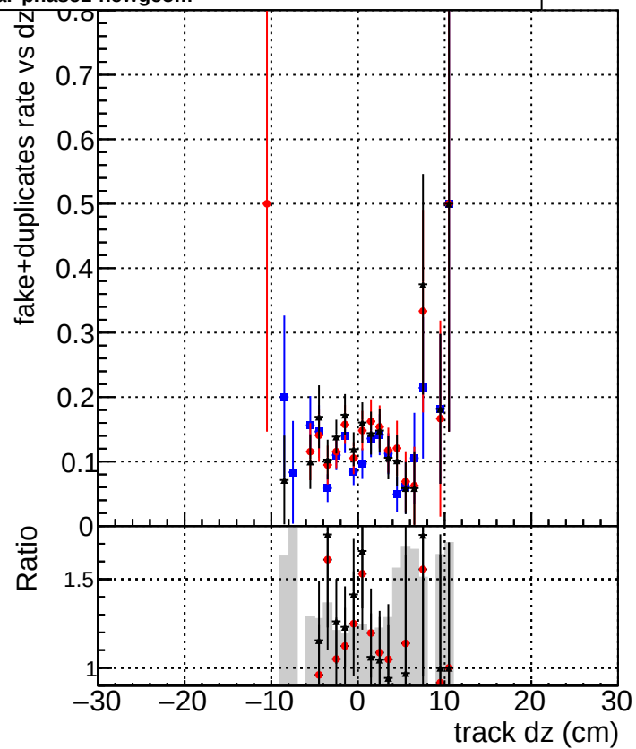
DQM_original_step2_ttbar-phase1-newgeom DQM_pixelCPE_step2_ttbar-phase1-newgeom DQM_pixelCPEChi2OR2_step2_ttbar-phase1-newgeom
