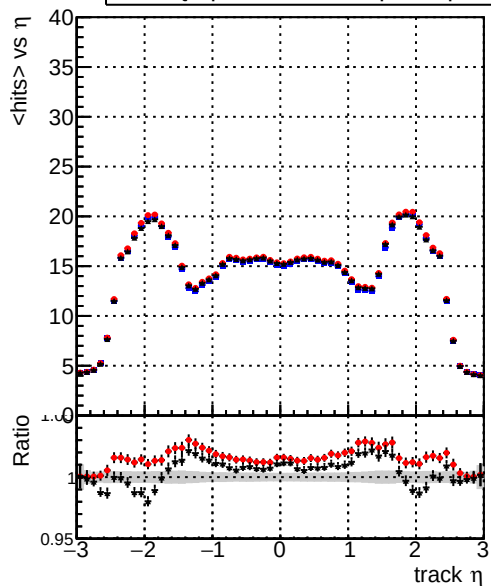
mean hits Legend: DQM_original_step2_ttbar-phase1-newgeom (blue line) DQM_pixelCPE_step2_ttbar-phase1-newgeom (red line) DQM_pixelCPEChi2OR2_step2_ttbar-phase1-newgeom (black line)
