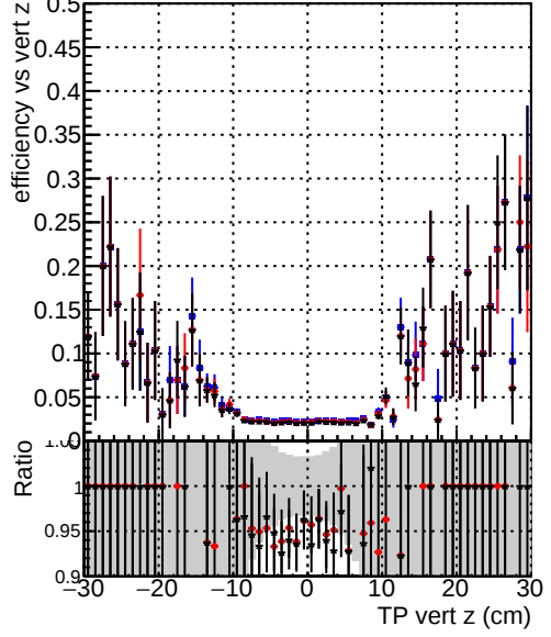
Efficiency vs. sim PV z —●— DQM_original_step2_ttbar-phase1-newgeom —●— DQM_pixelCPE_step2_ttbar-phase1-newgeom —●— DQM_pixelCPEChi2OR2_step2_ttbar-phase1-newgeom
