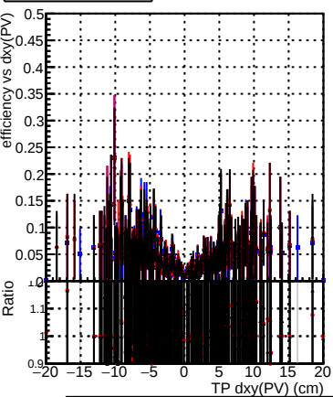
Efficiency vs Dxy(PV) Legend: DQM_original_step2_ttbar-phase1-newgeom (Blue line with circles) DQM_pixelCPE_step2_ttbar-phase1-newgeom (Red line with circles) DQM_pixelCPENoMatR_step2_ttbar-phase1-newgeom (Black line with circles)
