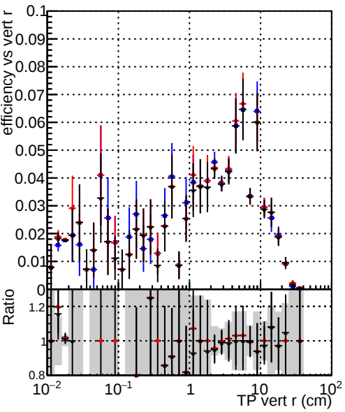
Efficiency vs vertpos DQM_original_step2_ttbar-phase1-newgeom DQM_pixelCPE_step2_ttbar-phase1-newgeom DQM_pixelCPENoMatR_step2_ttbar-phase1-newgeom
