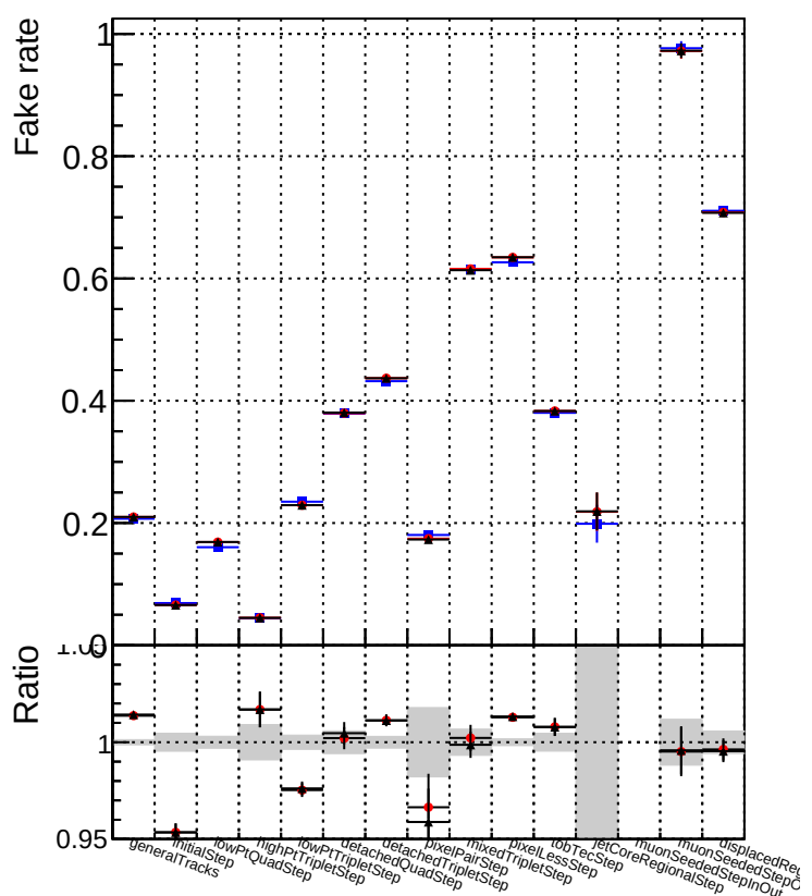
Fakerate vs collection
