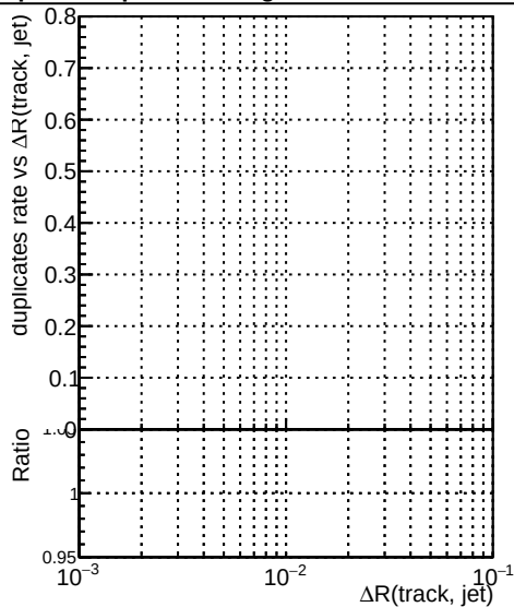
— \Delta R original step2 ttbar-phase1-newgeom — \Delta R pixelCPE step2 ttbar-phase1-newgeom — \Delta R pixelCPENoMatR step2 ttbar-phase1-newgeom
