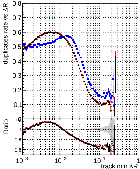
— \Delta R original step2 ttbar-phase1-newgeom — \Delta R pixelCPE step2 ttbar-phase1-newgeom — \Delta R pixelCPENoMatR step2 ttbar-phase1-newgeom
