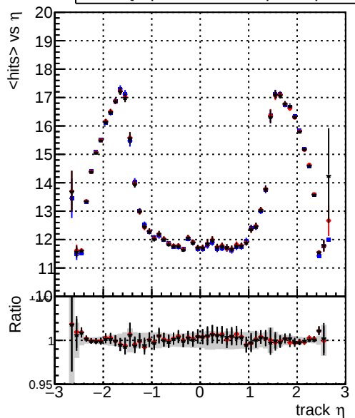
mean hits — DQM_original_step2_ttbar-phase1-newgeom — DQM_pixelCPE_step2_ttbar-phase1-newgeom — DQM_pixelCPENoMatR_step2_ttbar-phase1-newgeom
