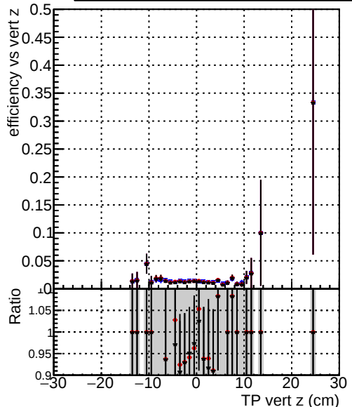
Efficiency vs vert z —●— DQM_original_step2_ttbar-phase1-newgeom —●— DQM_pixelCPE_step2_ttbar-phase1-newgeom —●— DQM_pixelCPENoMatR_step2_ttbar-phase1-newgeom
