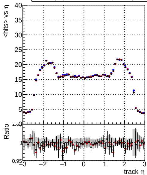
mean hits — DQM_original_step2_ttbar-phase1-newgeom — DQM_pixelCPE_step2_ttbar-phase1-newgeom — DQM_pixelCPENoMatR_step2_ttbar-phase1-newgeom
