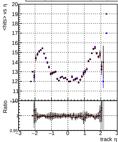
mean hits vs \eta — DQM_original_step2_ttbar-phase1-newgeom — DQM_pixelCPE_step2_ttbar-phase1-newgeom — DQM_pixelCPENoMatR_step2_ttbar-phase1-newgeom
