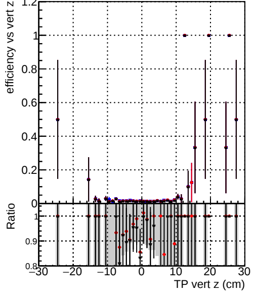
Efficiency vs. sim PV z —●— DQM_original_step2_ttbar-phase1-newgeom —●— DQM_pixelCPE_step2_ttbar-phase1-newgeom —●— DQM_pixelCPENoMatR_step2_ttbar-phase1-newgeom
