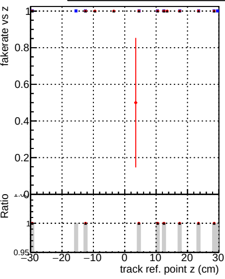
Legend: - DQM_original_step2_ttbar-phase1-newgeom (blue line with dots) - DQM_pixelCPE_step2_ttbar-phase1-newgeom (red line with dots) - DQM_pixelCPENoMatR_step2_ttbar-phase1-newgeom (black line with dots)
