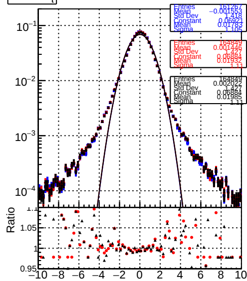
BDM original step2 tbar-phase-newgeom BDM pixelCFEnomatr step2 tbar-phase-newgeom
