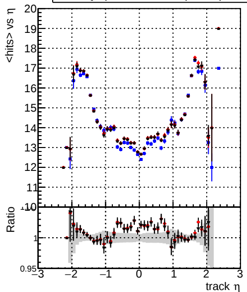
mean hits vs \eta — DQM_original_step2_ttbar-phase1-newgeom — DQM_pixelCPE_step2_ttbar-phase1-newgeom — DQM_pixelCPENoMatR_step2_ttbar-phase1-newgeom
