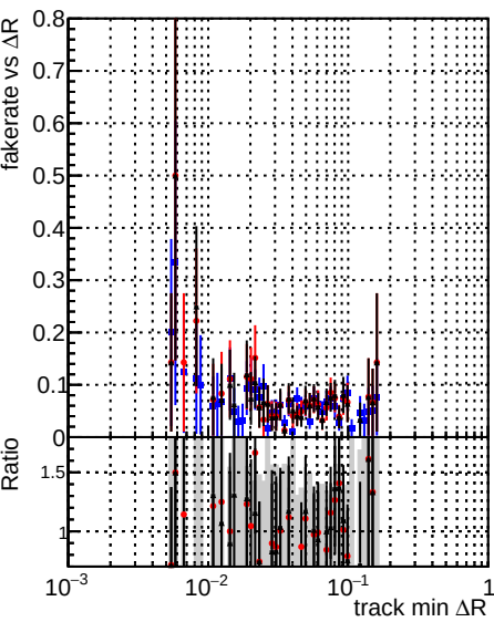
Fake rate vs \Delta R(\text{track, jet}) Legend: DQM original step2 ttbar-phase1-newgeom (blue squares) DQM pixelCPE step2 ttbar-phase1-newgeom (red circles) DQM pixelCPENoMatR step2 ttbar-phase1-newgeom (black crosses)
