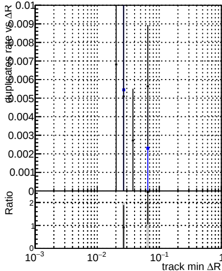
— DQM_original_step2_ttbar-phase1-newgeom — DQM_pixelCPE_step2_ttbar-phase1-newgeom — DQM_pixelCPENoMatR_step2_ttbar-phase1-newgeom
